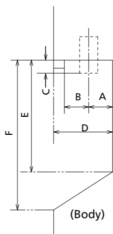
Sectional view of terminal b
