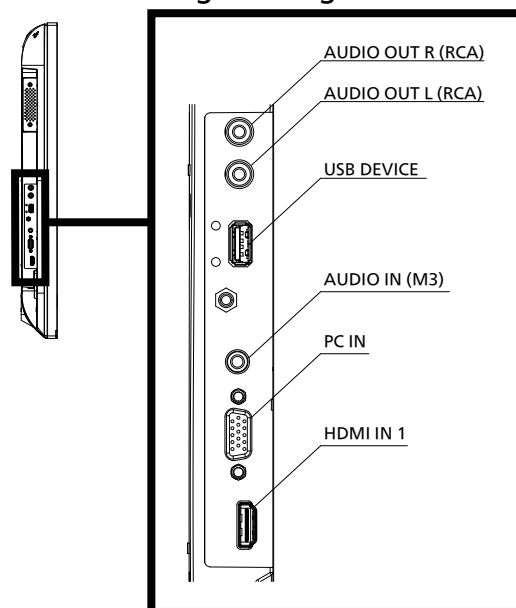
Magnified figure of terminal b
