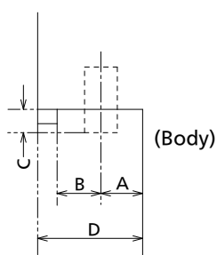
Sectional view of terminal b
