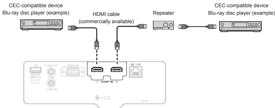
Connection example with CEC-compatible device
