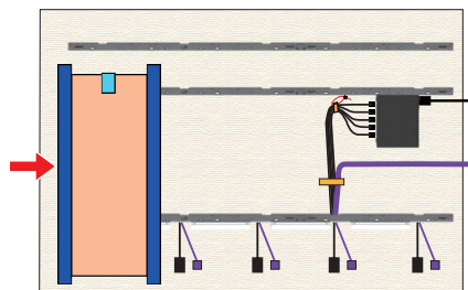
Cabinet module rear view
