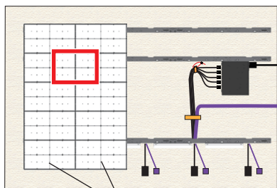
Cabinet module (TY-FD15AS5)
