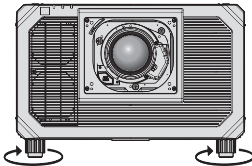
Maximum adjustable range Adjustable feet: 20 mm (25/32") each
