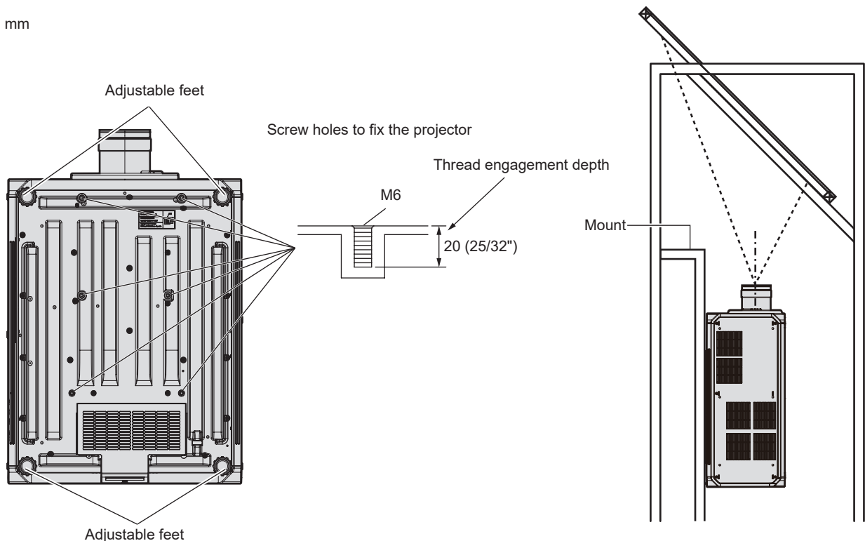
Positions of screw holes to fix projector and adjustable feet
