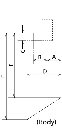
Sectional view of terminal a (SERIAL IN / LAN / HDMI IN 2 / HDMI IN 3)
