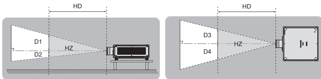
Example of using ET-D3LES250
