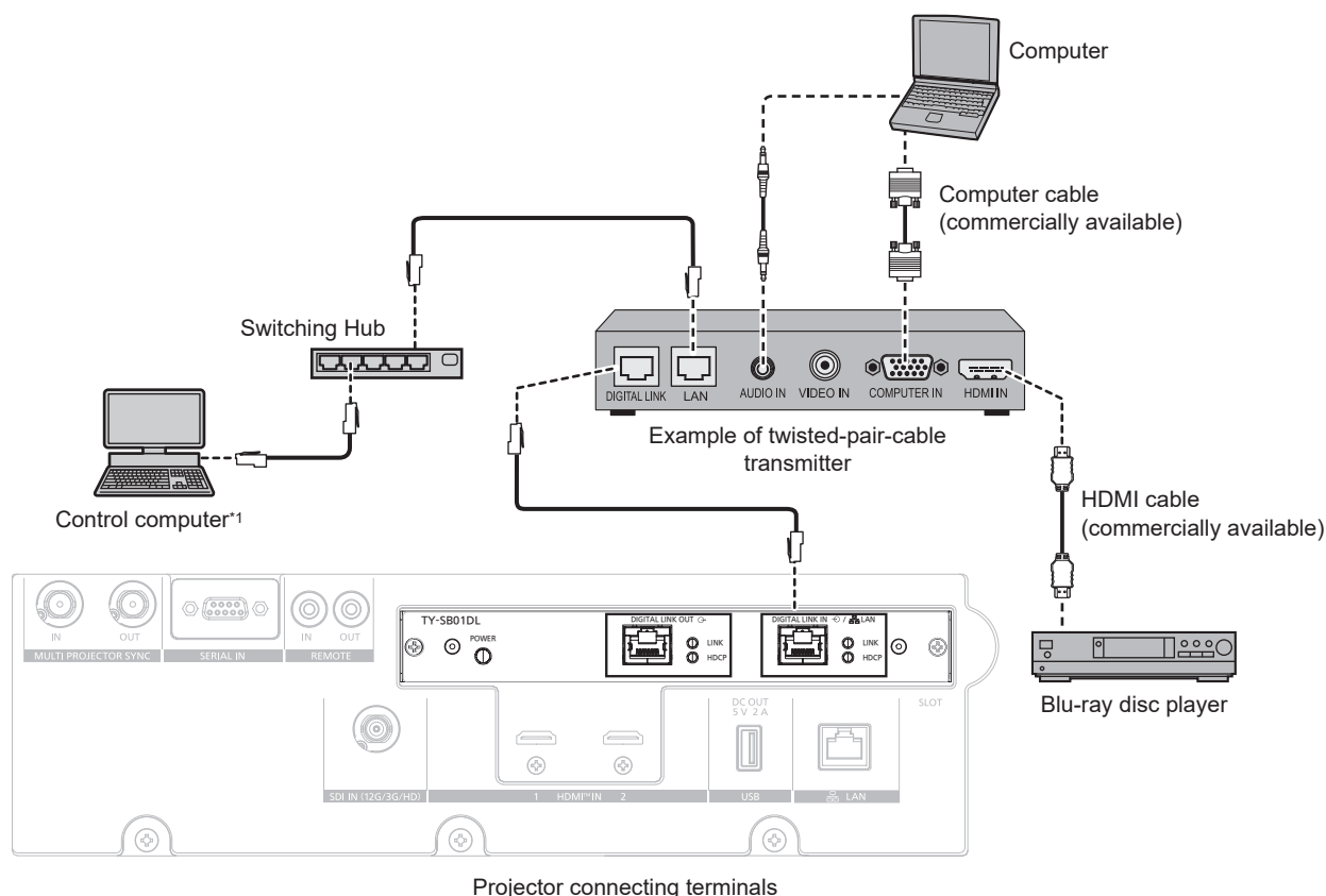
Projector connecting terminals
